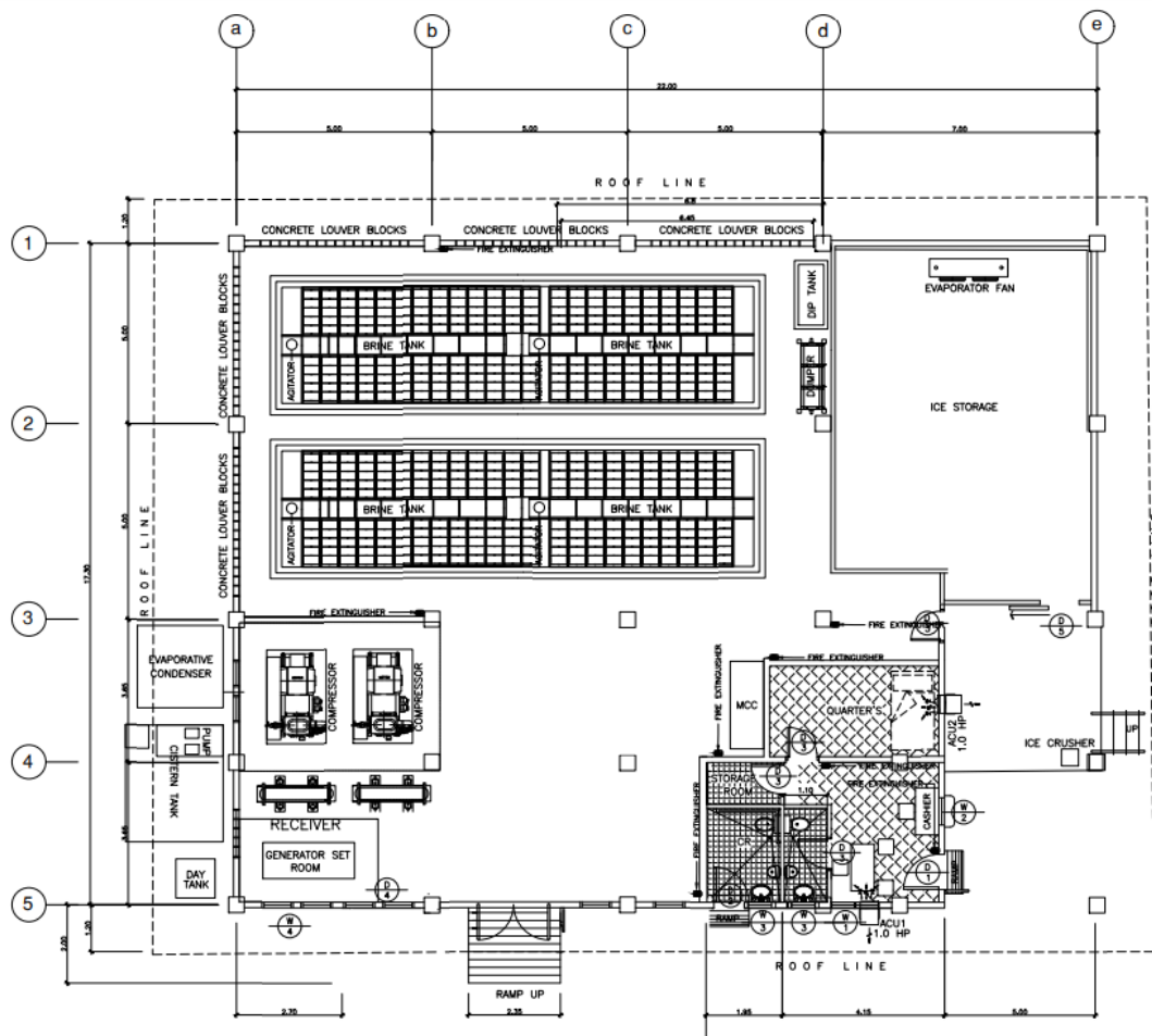
ICE PLANT AND ICE STORAGE EQUIPMENT PLAN SCALE 1:150 MTS.
