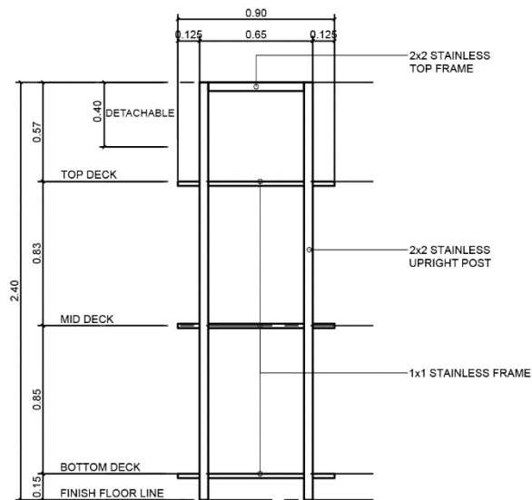
2 A 1 NTS: STAINLESS STORAGE RACK SPOT DETAIL
