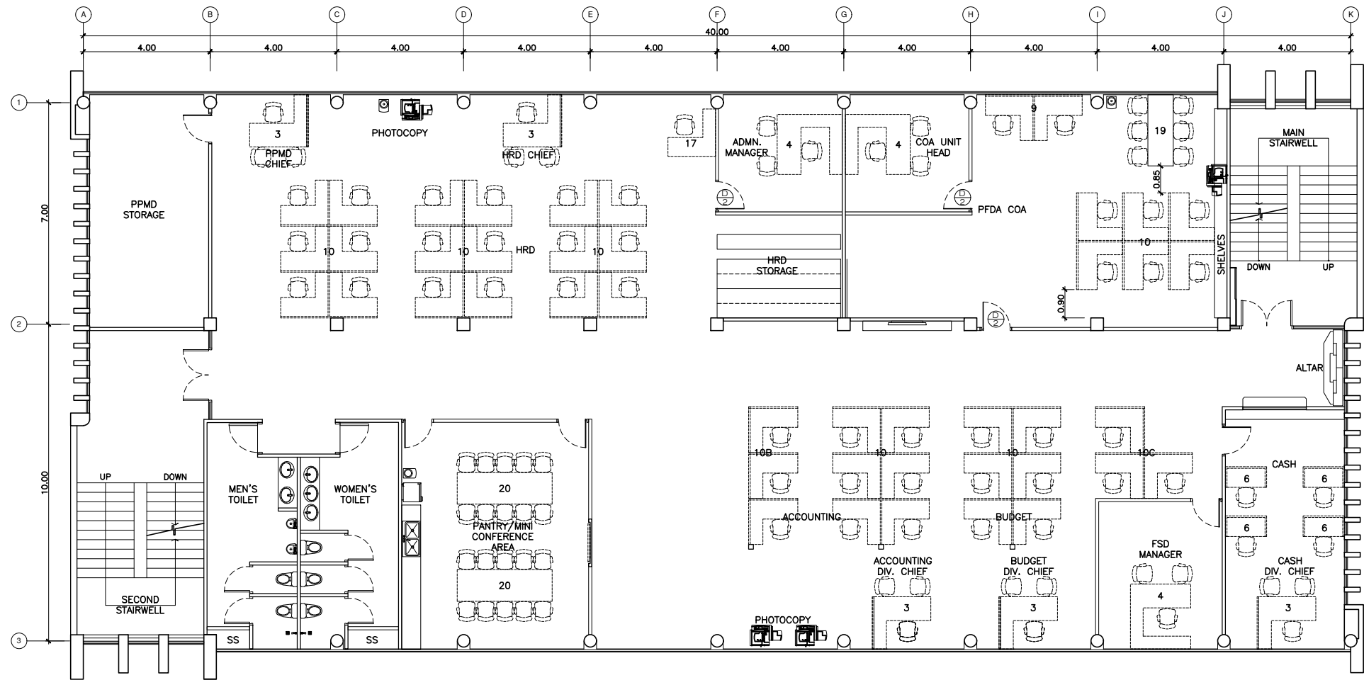
PROPOSED THIRD FLOOR PLAN SCALE 1:100 MTS.
