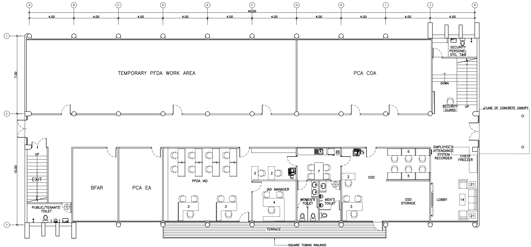
PROPOSED GROUND FLOOR PLAN SCALE 1:100 MTS.
