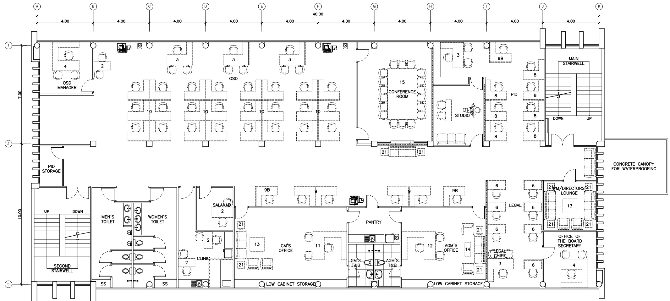
PROPOSED SECOND FLOOR PLAN SCALE 1:100 MTS.
